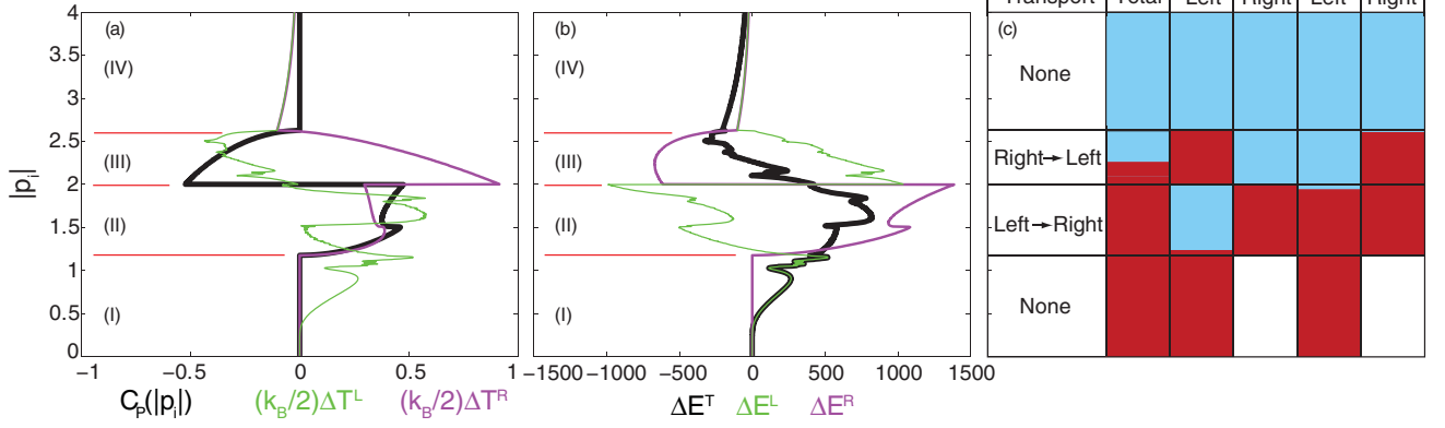
FIG. 1. (Color online) (a) Net particle transport, C_P(|p_i|) (thickest curve), and the change in average energy per particle in the left reservoir, (k_B/2)\Delta T^L(|p_i|) [thin (green) curve] and right reservoir, (k_B/2)\Delta T^R(|p_i|) [medium (purple) curve]. When C_P(|p_i|) is positive (negative) there is net particle transport from left to right (right to left). When (k_B/2)\Delta T^{L,R}(|p_i|) is positive (negative), the pump increases (decreases) the average energy of particles scattered into the respective reservoir, and the temperature in that reservoir increases (decreases). (b) Total energy change in both reservoirs, \Delta E^T(|p_i|) (thickest curve), in the left reservoir, \Delta E^L(|p_i|) [thin (green) curve], and in the right reservoir, \Delta E^R(|p_i|) [medium (purple) curve]. When \Delta E^T(|p_i|) is positive, the pumps adds net energy to the reservoirs; when negative, the reservoirs lose net energy to the pump. When \Delta E^{L,R}(|p_i|) is positive (negative), the pump increases (decreases) the total energy in the respective reservoir. (c) Summary of (a) and (b). Dark gray (red) indicates an increase, and light gray (blue) represents a decrease. No color is plotted if the quantity does not change.
