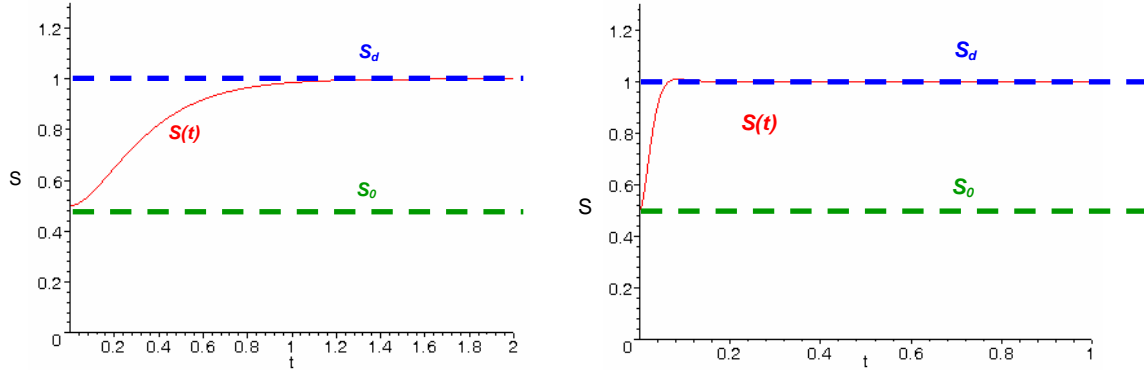
Figure 4: Time-evolution of a generic system with PI control feedback for S_0=0.5 and S_d=1 . For the left hand plot the gain parameters are g_p=-10 , g_I=-30 , while for the right hand plot the parameters are g_p=-100 , g_I=-4000 . The small overshoot in the left hand plot is due to a small imaginary part in the exponential exponent of equation 11(a).
